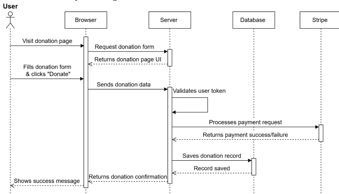
Figure 3 Online Donation Sequence Diagram
