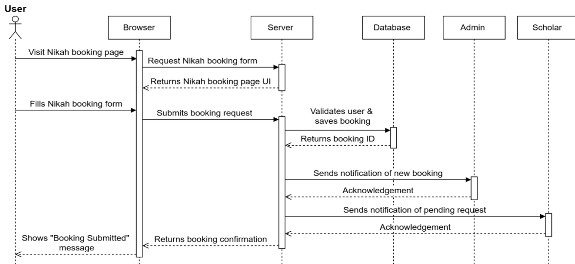
Figure 4 Nikah Booking Sequence Diagram
