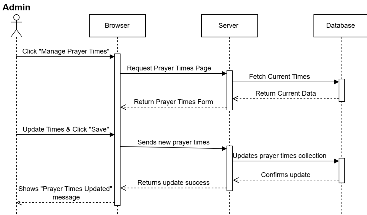
Figure 5 Admin Update Prayer Times Sequence Diagram
