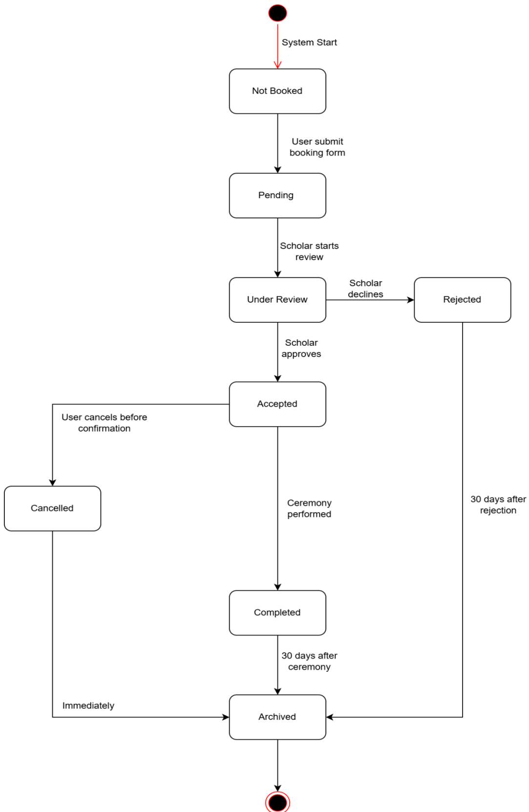
Figure 7 Nikah Booking Status State Diagram
